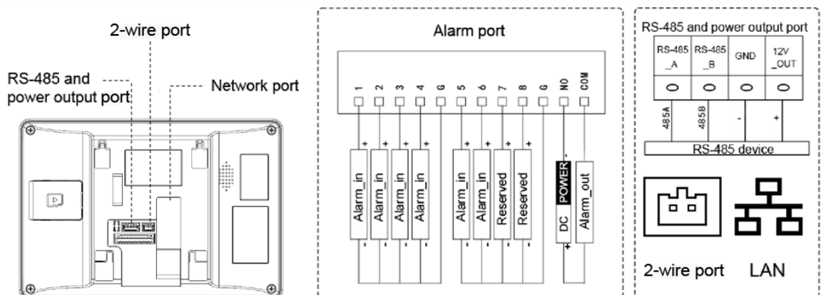
Figure 1-2 Rear panel for 2-wire model
