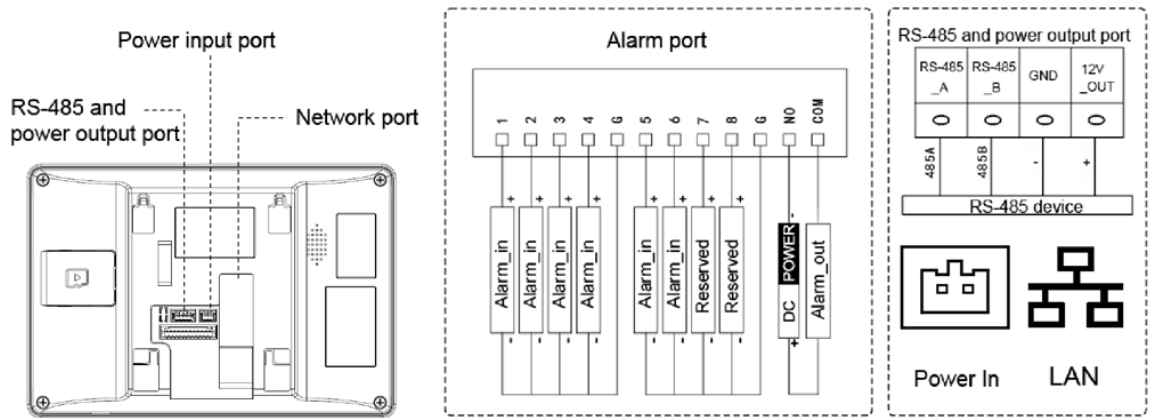
Figure 1-3 Rear panel for non 2-wire model
