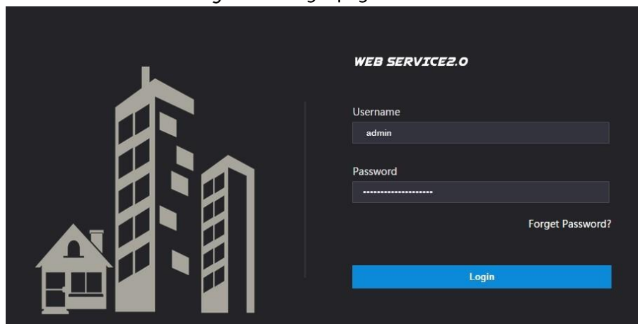
Figure 3-4 Login page
